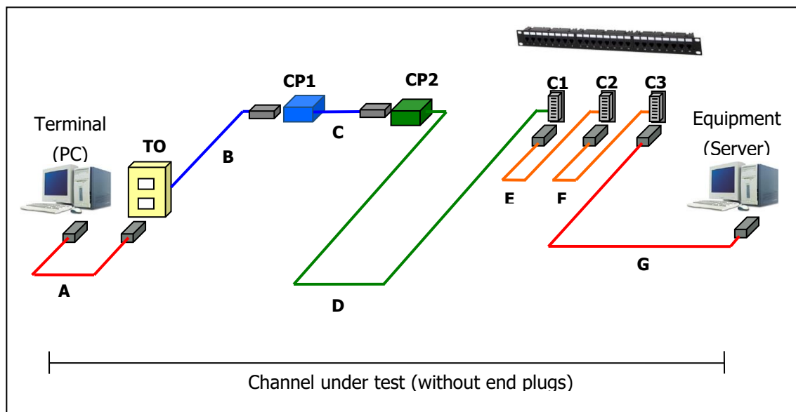
Figure 1. Channel definition (4 connector model).
